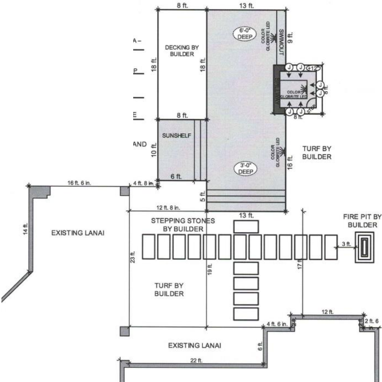
Pool Design
